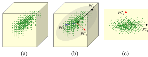
Figure 1: Illustration of principal component analysis. High-dimensional data (a) plotted with respect to their first three Principal Components (PCs) (b) and first two PCs (c).
