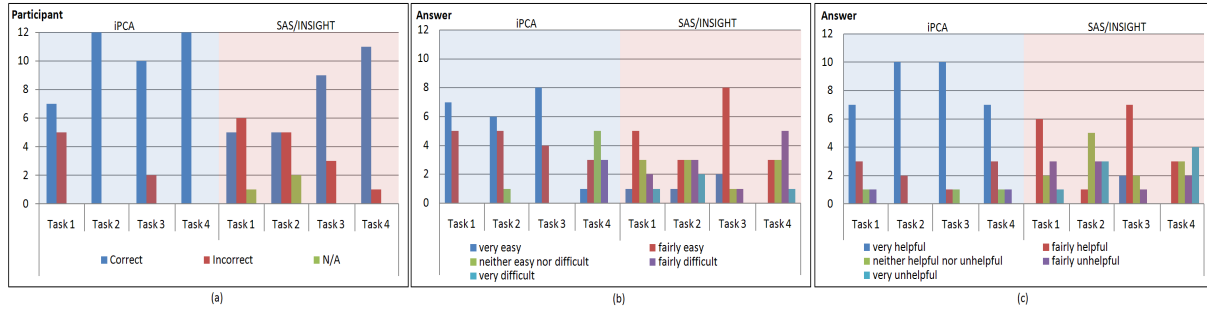
Figure 3: Participants’ accuracy in solving each task (a) and the results of a post-task questionnaire performed right after solving each task - (b) difficulty of the task and (c) helpfulness of the system in solving the task.
